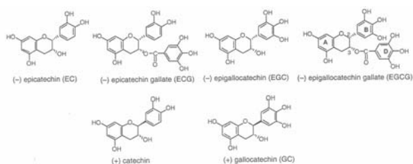
Fig. 1. Structures of the major polyphenolic catechins present in green tea.
